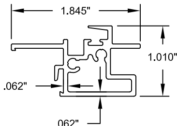
9 STD. MEETING RAIL 6063-T6 ALUMINUM
