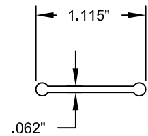
12 DOGBONE REINFORCEMENT 6063-T6 ALUMINUM
