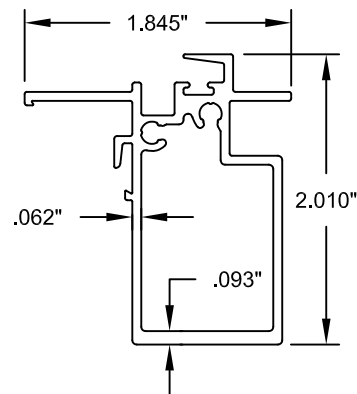
6 HD FIXED MEETING RAIL 6063-T6 ALUMINUM
