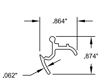
7 SIDE RAIL LOCK 6063-T6 ALUMINUM
