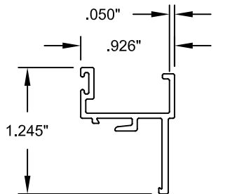
8 SASH TOP & BOTTOM RAIL 6063-T6 ALUMINUM
