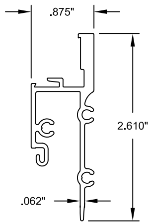
3 SILL ADAPTER 6063-T6 ALUMINUM
